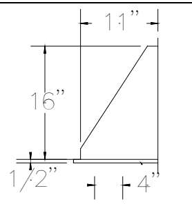
Bracket Detail
