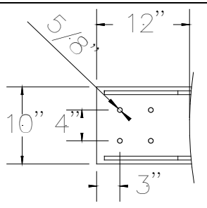
Bracket Detail
